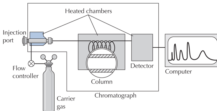
FIGURE 20.4 Schematic diagram of a gas chromatograph
