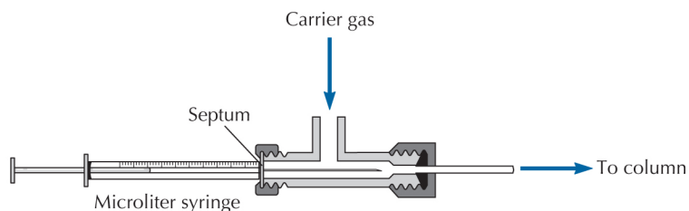
FIGURE 20.5 Injection port during sample injection.
