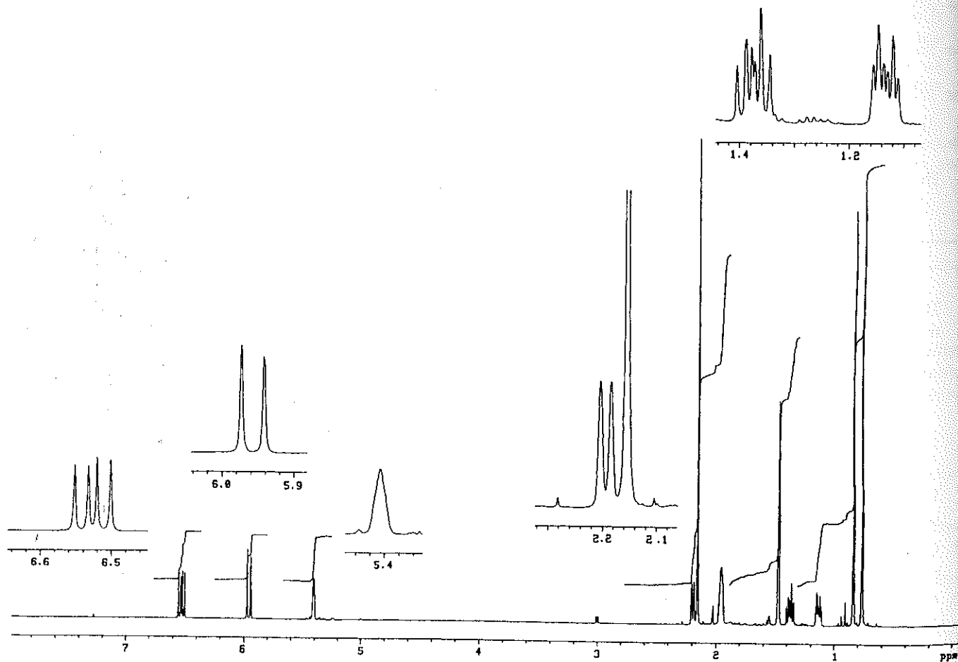
Figure 23.12 500-MHz ^1\text{H} -NMR spectrum of \alpha -ionone in \text{CDCl}_3 .
