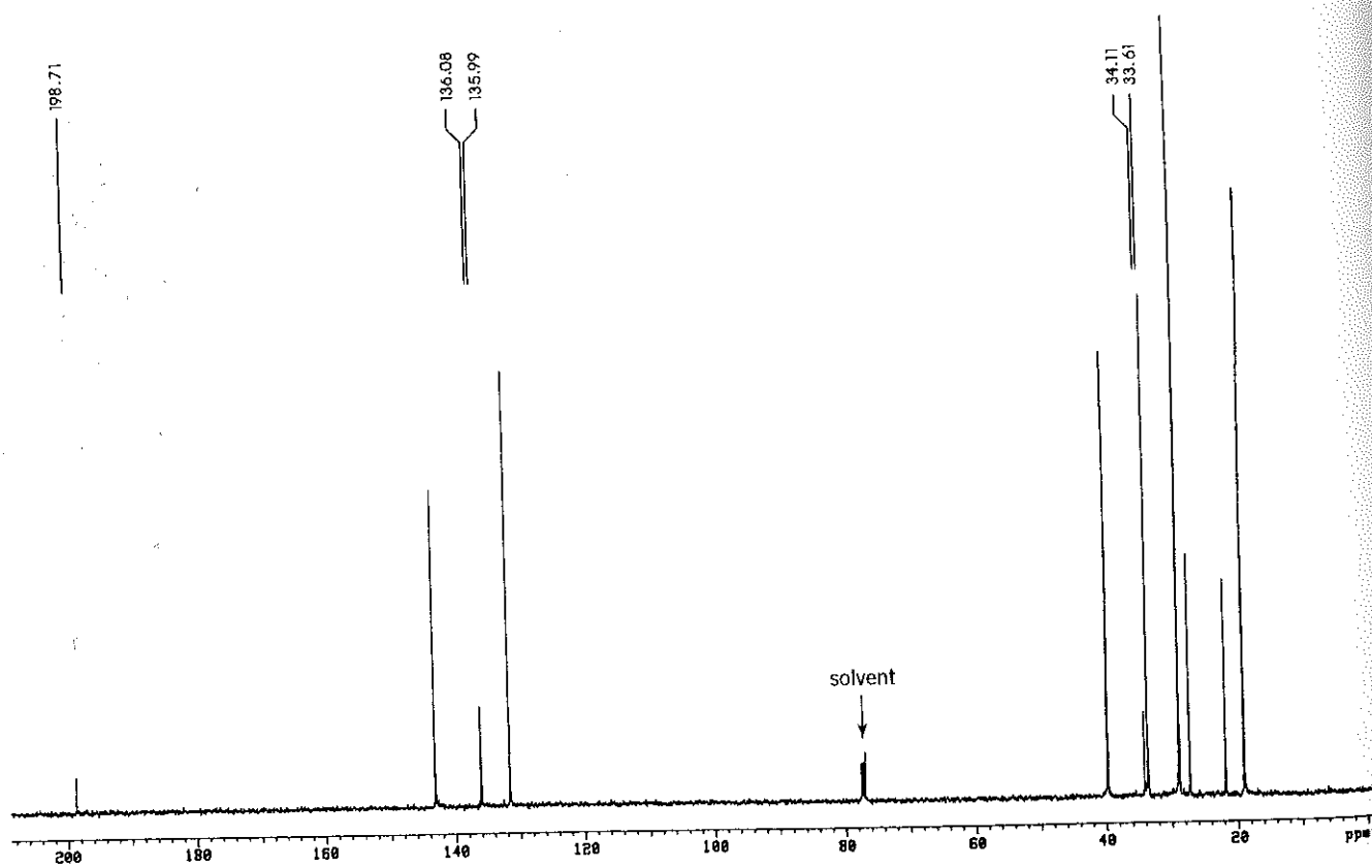
Figure 23.16 125.7-MHz 13 C-NMR spectrum of β-ionone in CDCl 3 .
