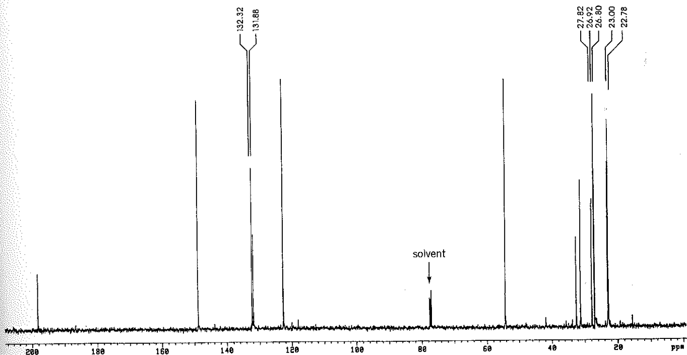
Figure 23.13 125.7-MHz ^{13}\text{C} -NMR spectrum of \alpha -ionone in \text{CDCl}_3 .
