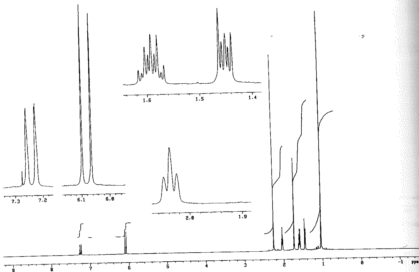
Figure 23.15 500-MHz 1 H-NMR spectrum of β-ionone in CDCl 3 .
