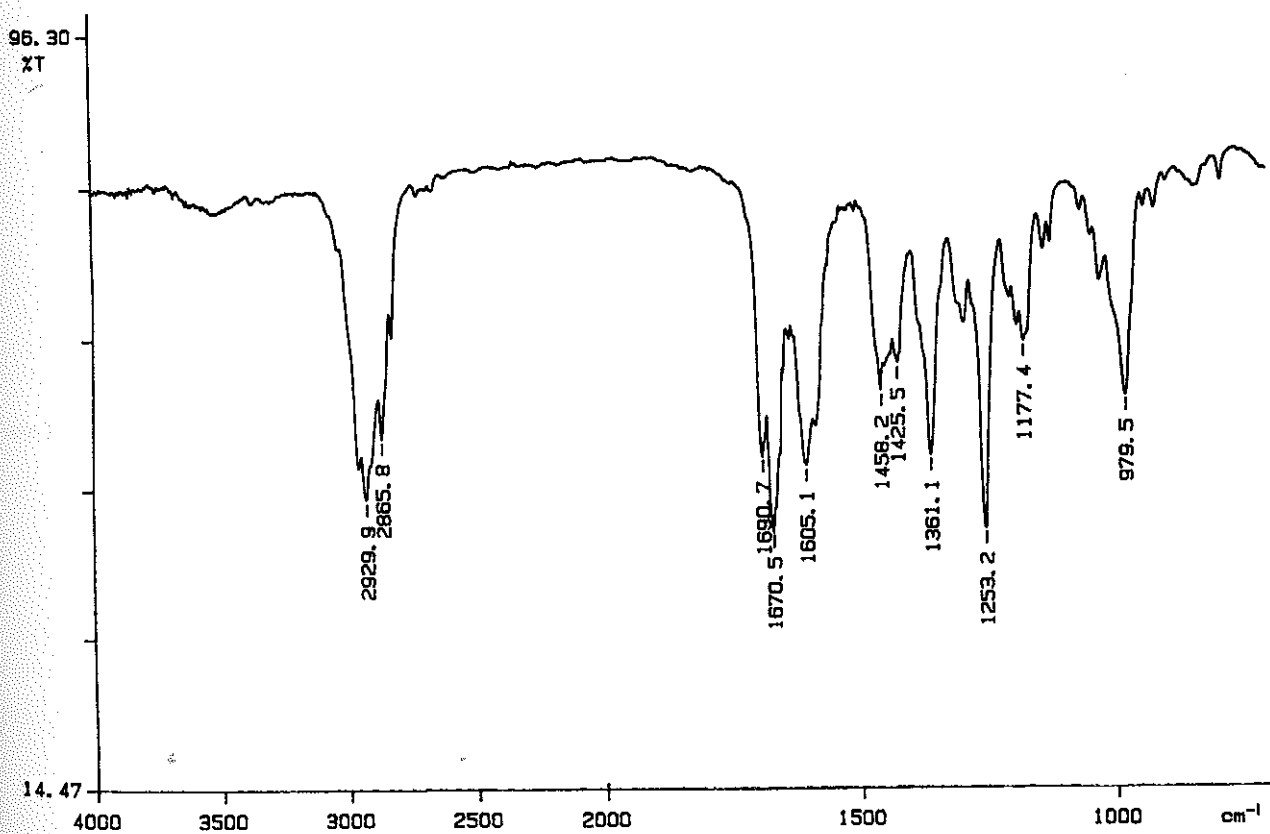
Figure 23.14 IR spectrum of \beta -ionone (neat).
