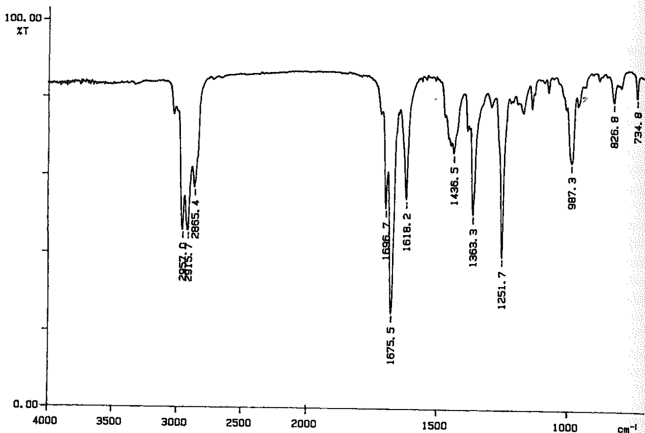
Figure 23.11 IR spectrum of \alpha -ionone (neat).
